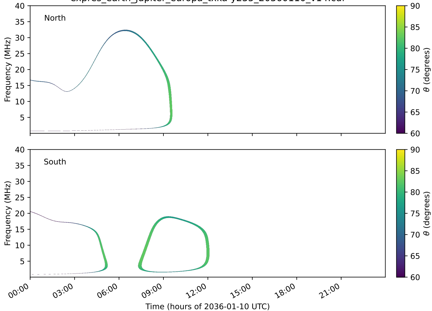
expres_earth_jupiter_europa_txka-y235_20360110_v14.cdf
