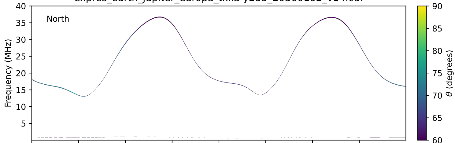
expres_earth_jupiter_europa_txka-y235_20360102_v14.cdf
