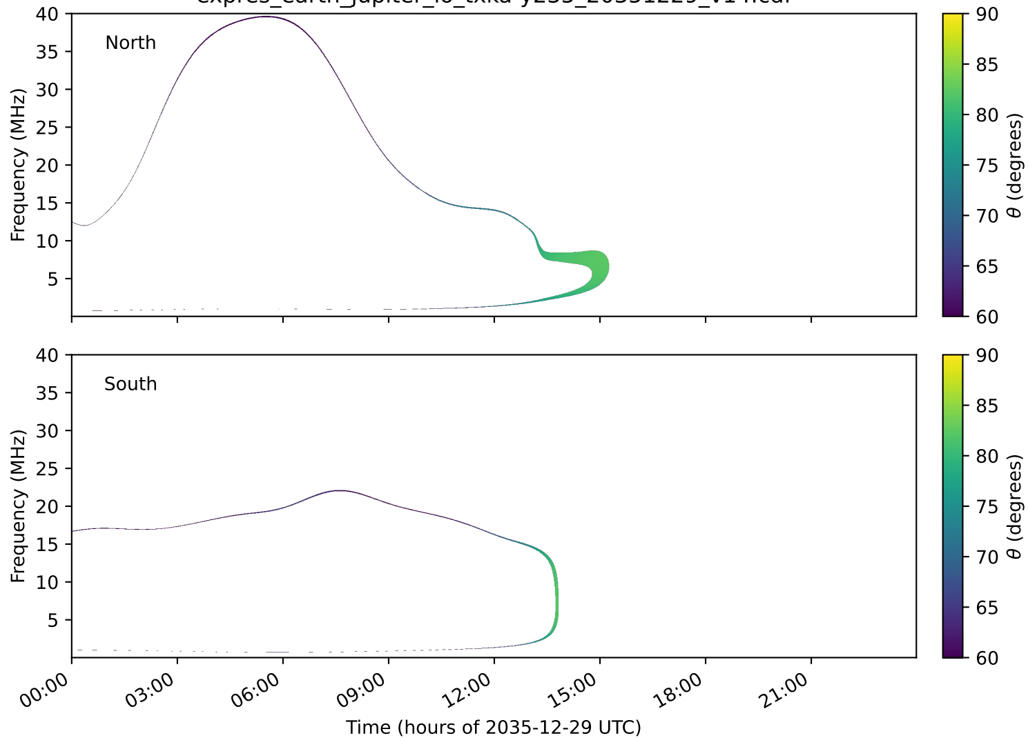
expres_earth_jupiter_io_txka-y235_20351229_v14.cdf
