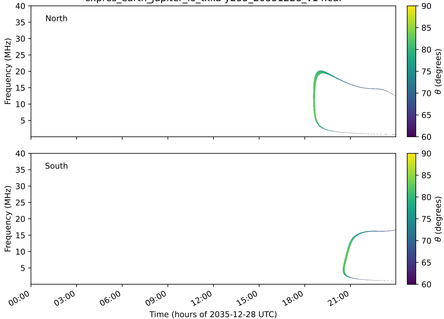
expres_earth_jupiter_io_txka-y235_20351228_v14.cdf
