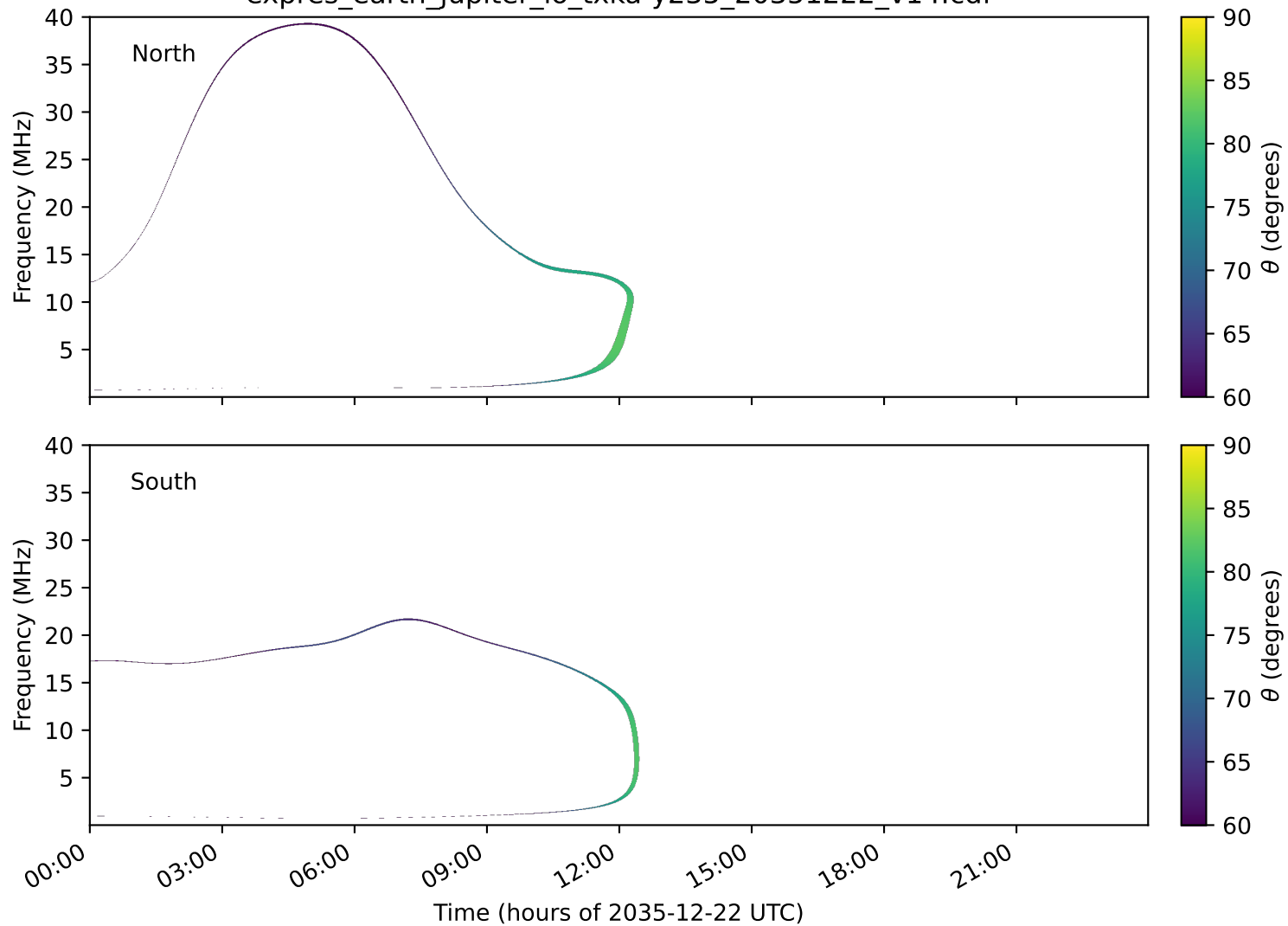
expres_earth_jupiter_io_txka-y235_20351222_v14.cdf
