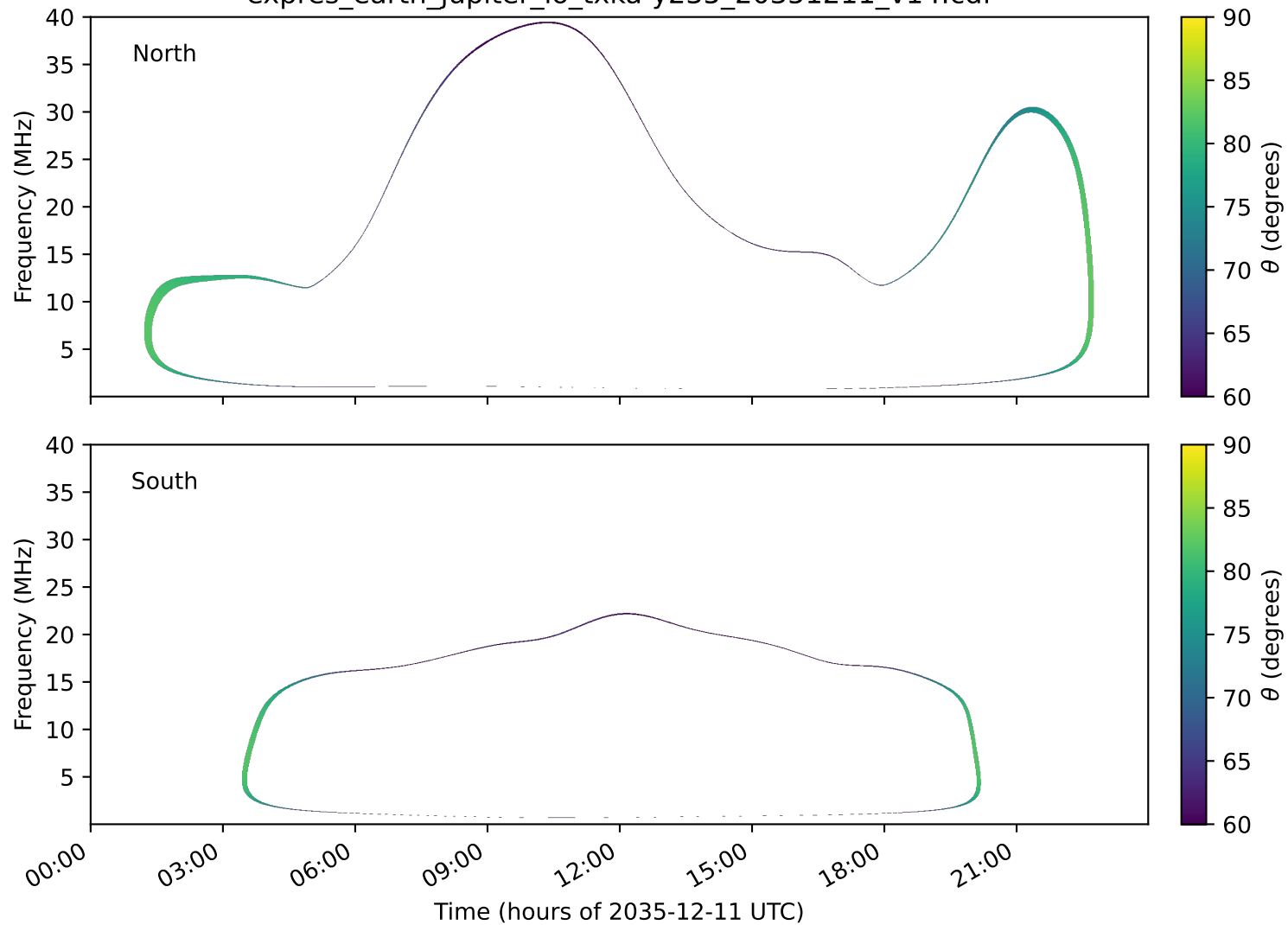
expres_earth_jupiter_io_txka-y235_20351211_v14.cdf
