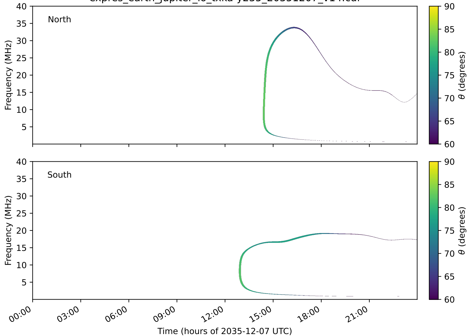
expres_earth_jupiter_io_txka-y235_20351207_v14.cdf
