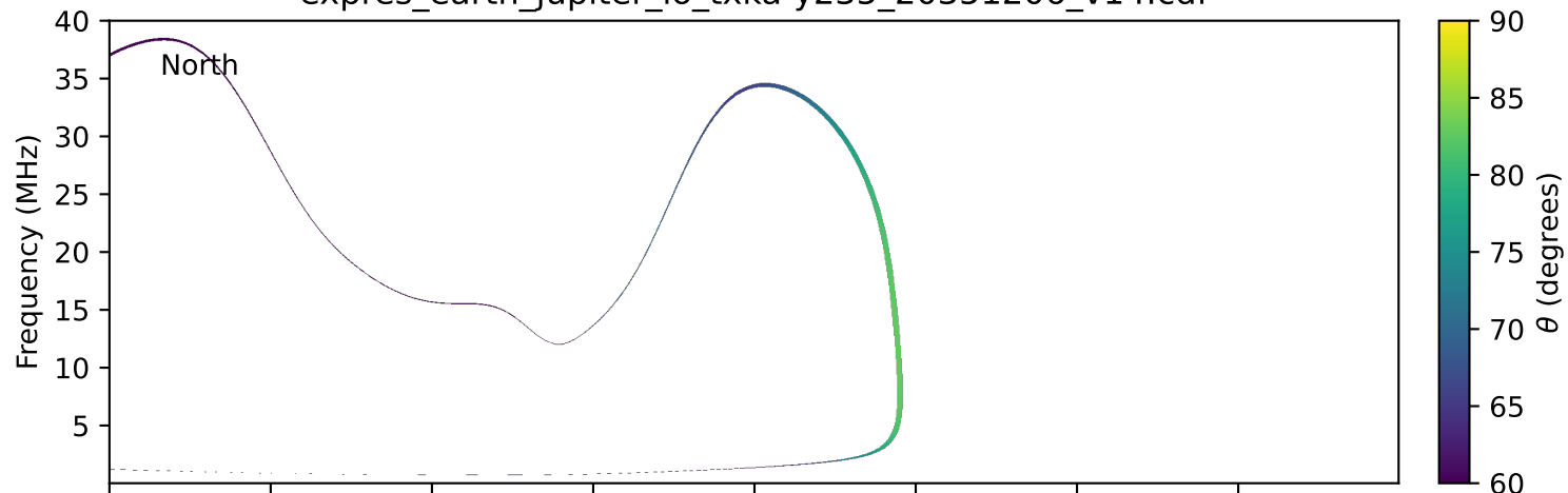
expres_earth_jupiter_io_txka-y235_20351206_v14.cdf
