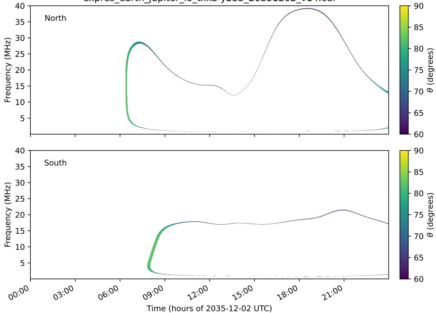
expres_earth_jupiter_io_txka-y235_20351202_v14.cdf
