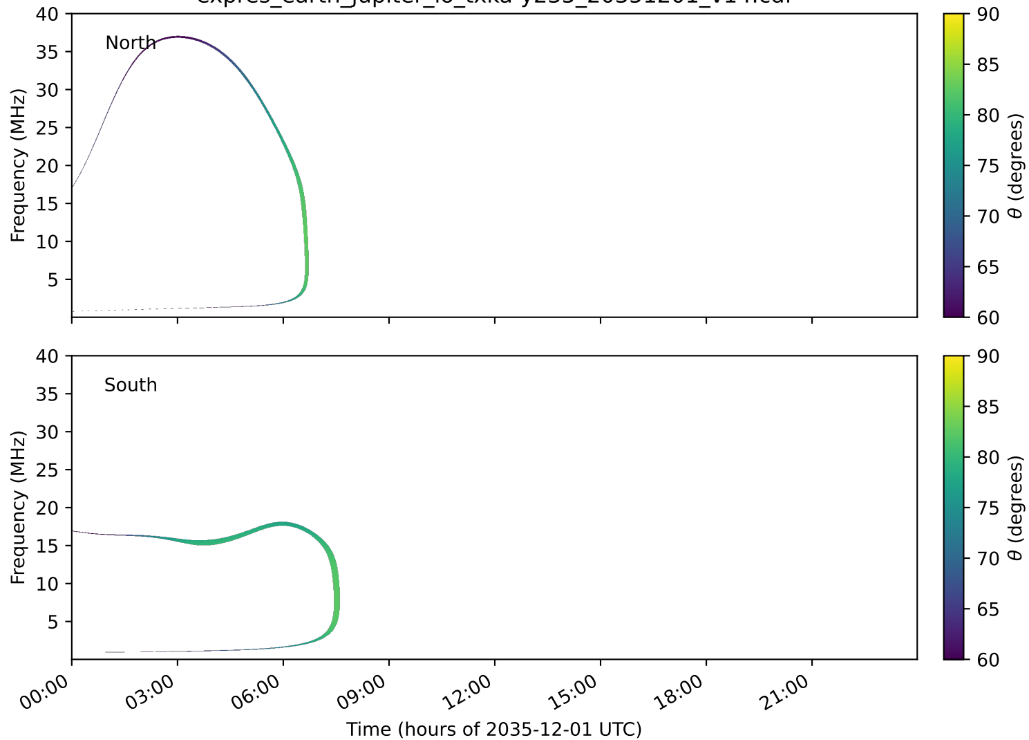
expres_earth_jupiter_io_txka-y235_20351201_v14.cdf
