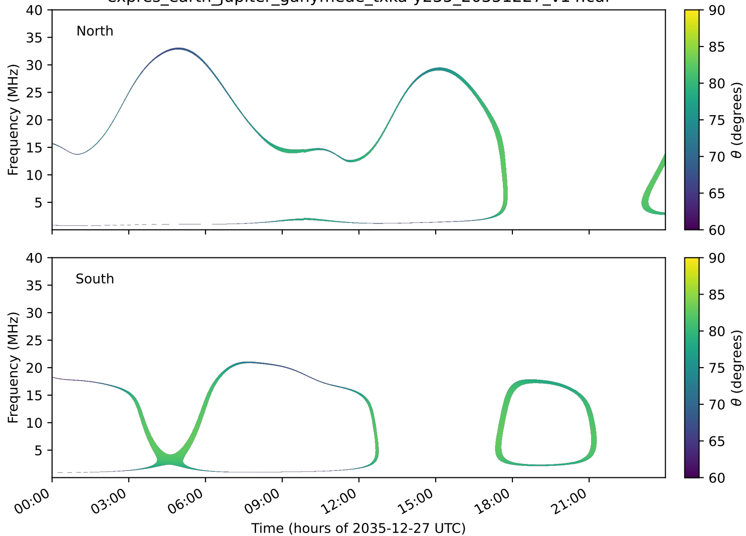
expres_earth_jupiter_ganymede_txka-y235_20351227_v14.cdf
