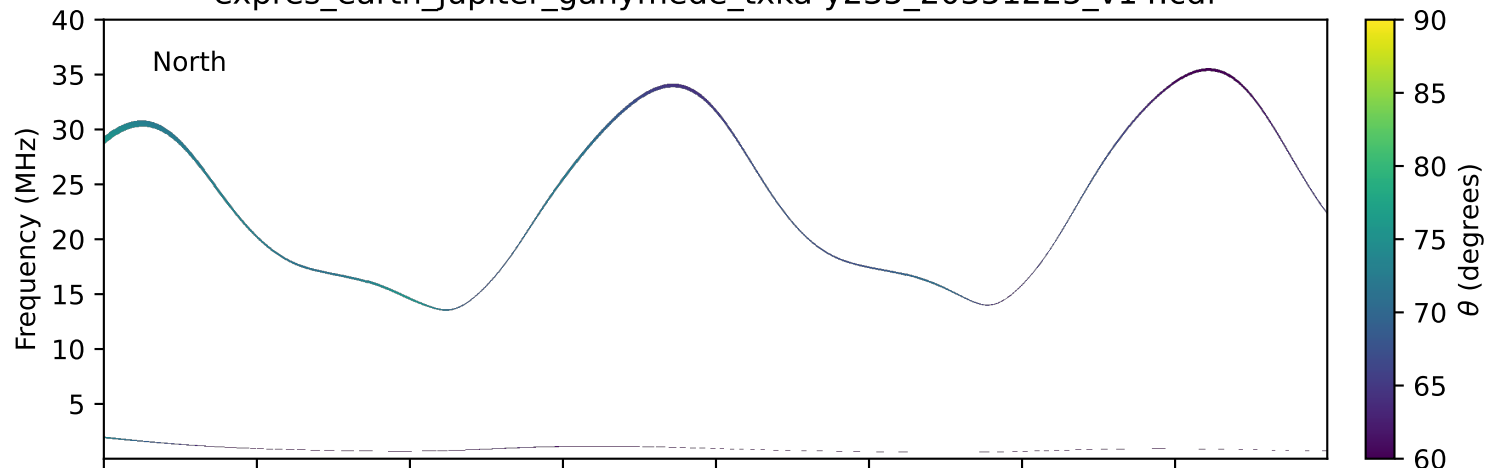
expres_earth_jupiter_ganymede_txka-y235_20351225_v14.cdf
