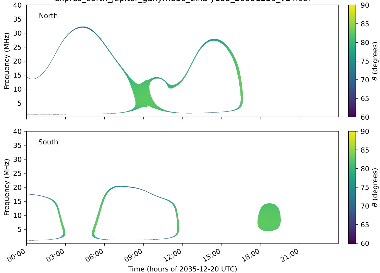
expres_earth_jupiter_ganymede_txka-y235_20351220_v14.cdf
