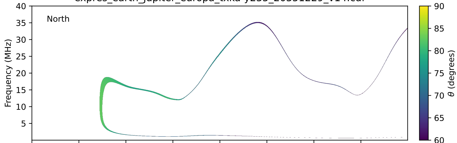
expres_earth_jupiter_europa_txka-y235_20351229_v14.cdf
