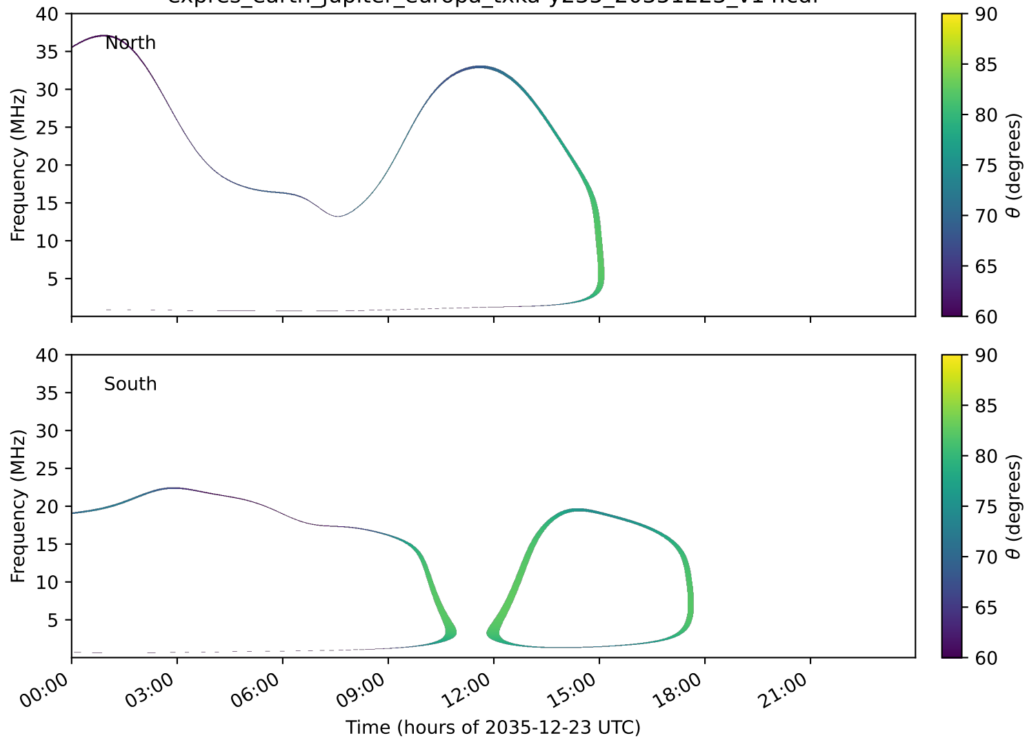
expres_earth_jupiter_europa_txka-y235_20351223_v14.cdf
