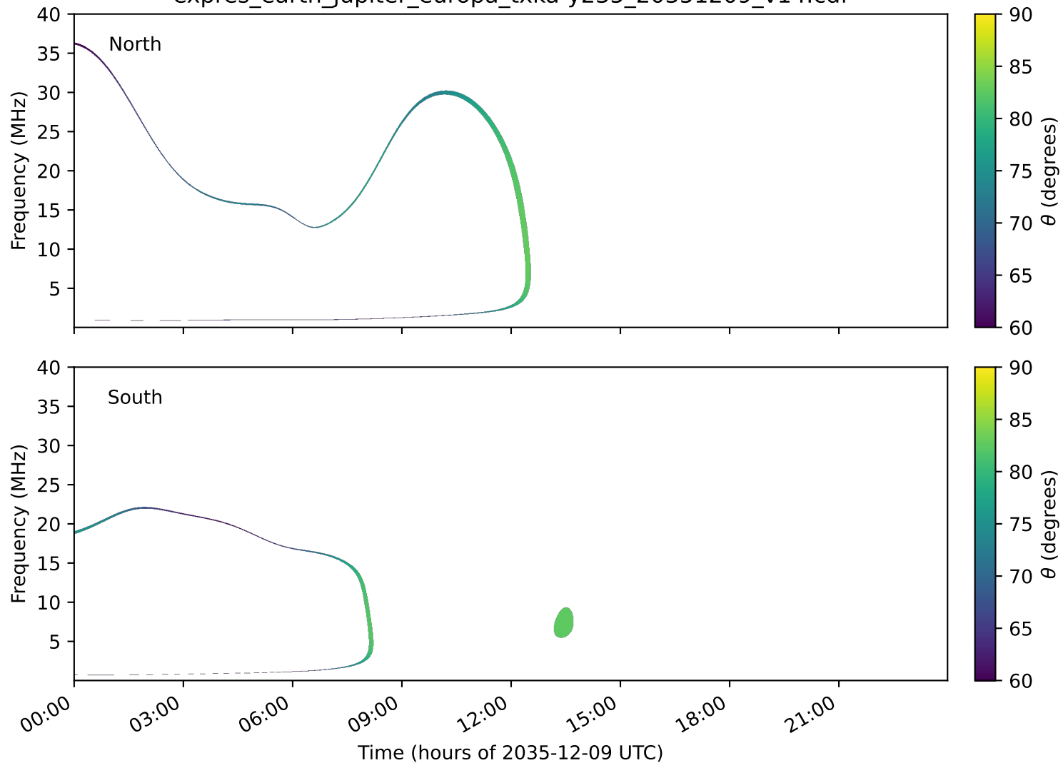
expres_earth_jupiter_europa_txka-y235_20351209_v14.cdf
