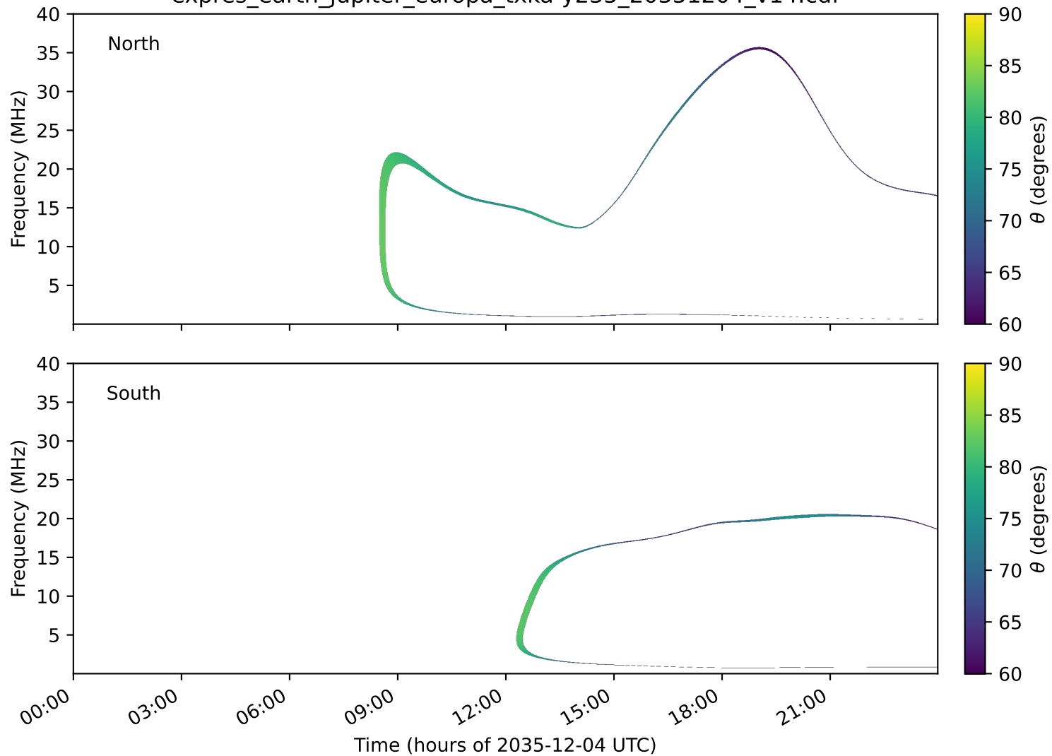
expres_earth_jupiter_europa_txka-y235_20351204_v14.cdf
