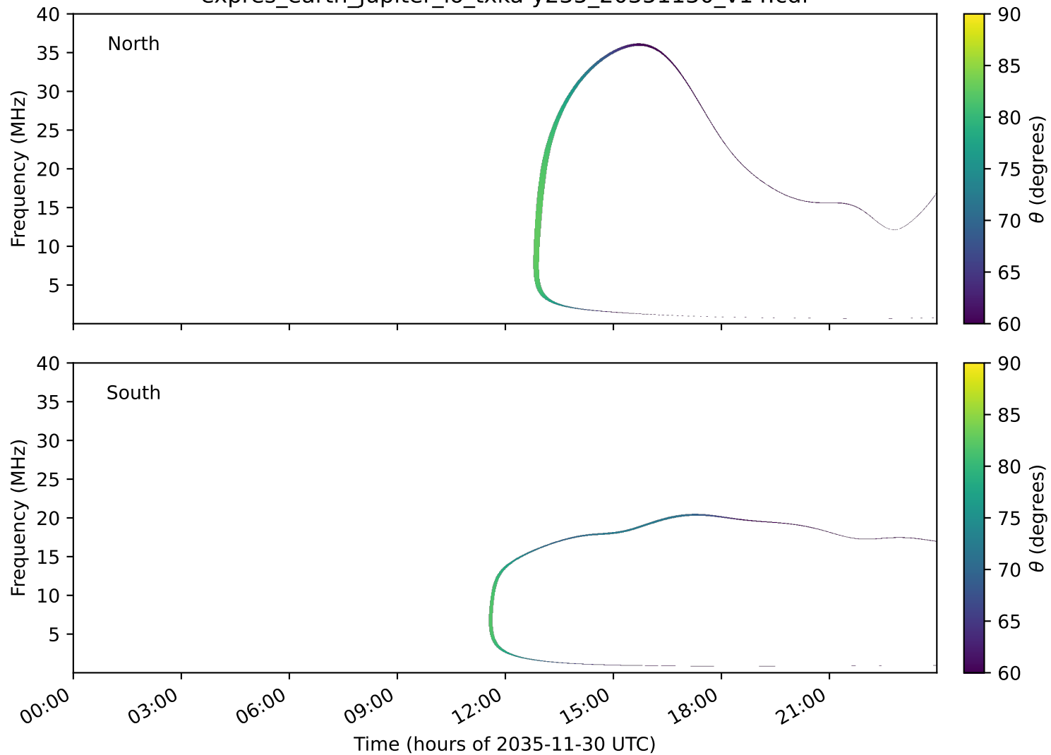
expres_earth_jupiter_io_txka-y235_20351130_v14.cdf
