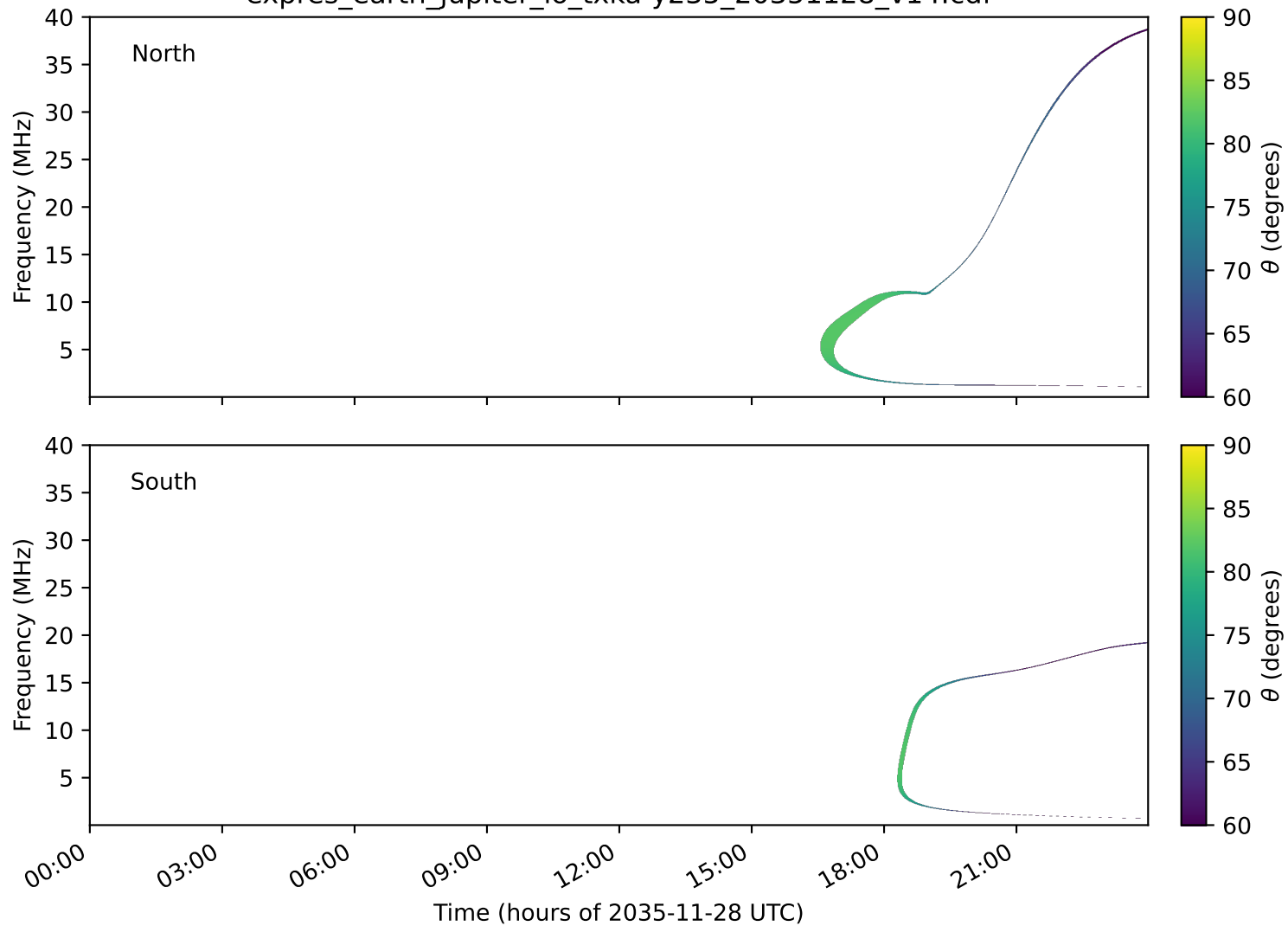
expres_earth_jupiter_io_txka-y235_20351128_v14.cdf
