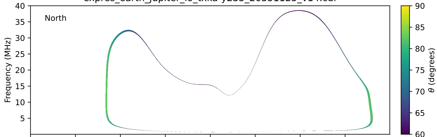
expres_earth_jupiter_io_txka-y235_20351125_v14.cdf
