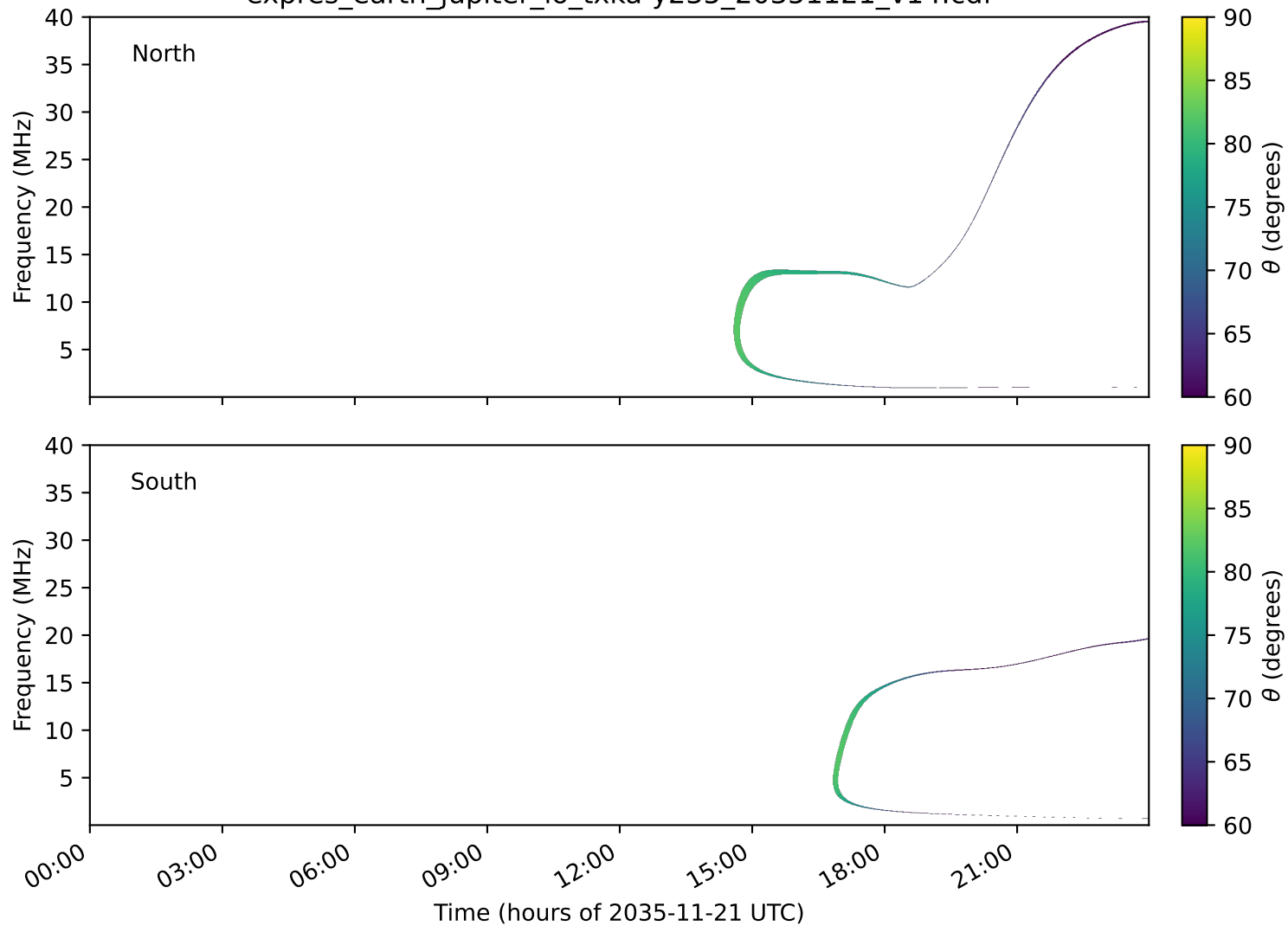
expres_earth_jupiter_io_txka-y235_20351121_v14.cdf
