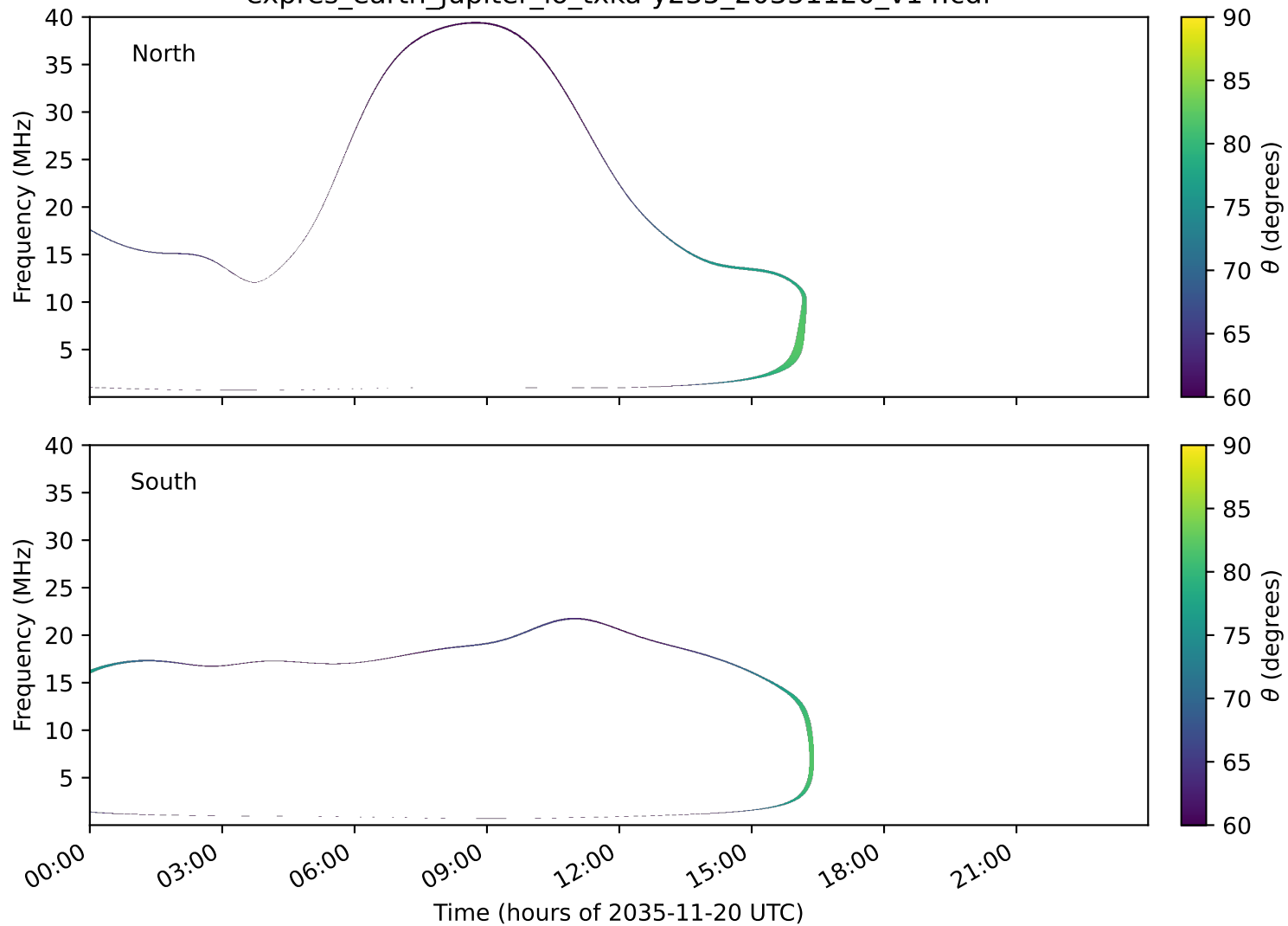
expres_earth_jupiter_io_txka-y235_20351120_v14.cdf
