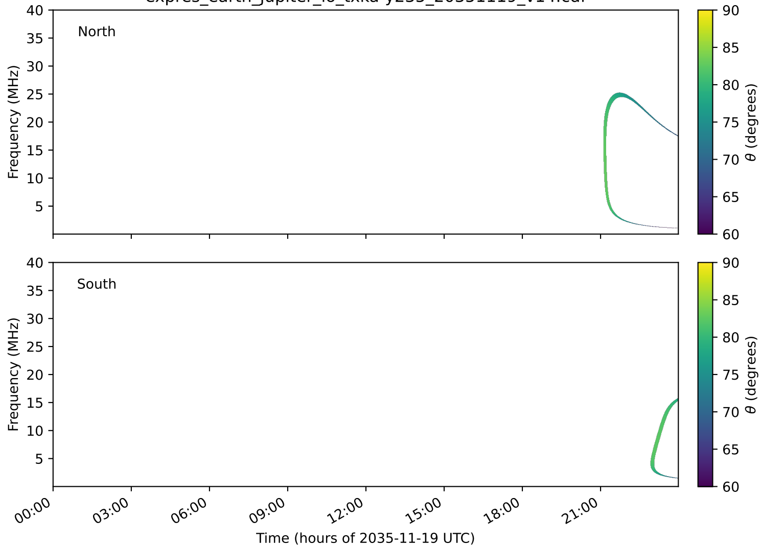
expres_earth_jupiter_io_txka-y235_20351119_v14.cdf
