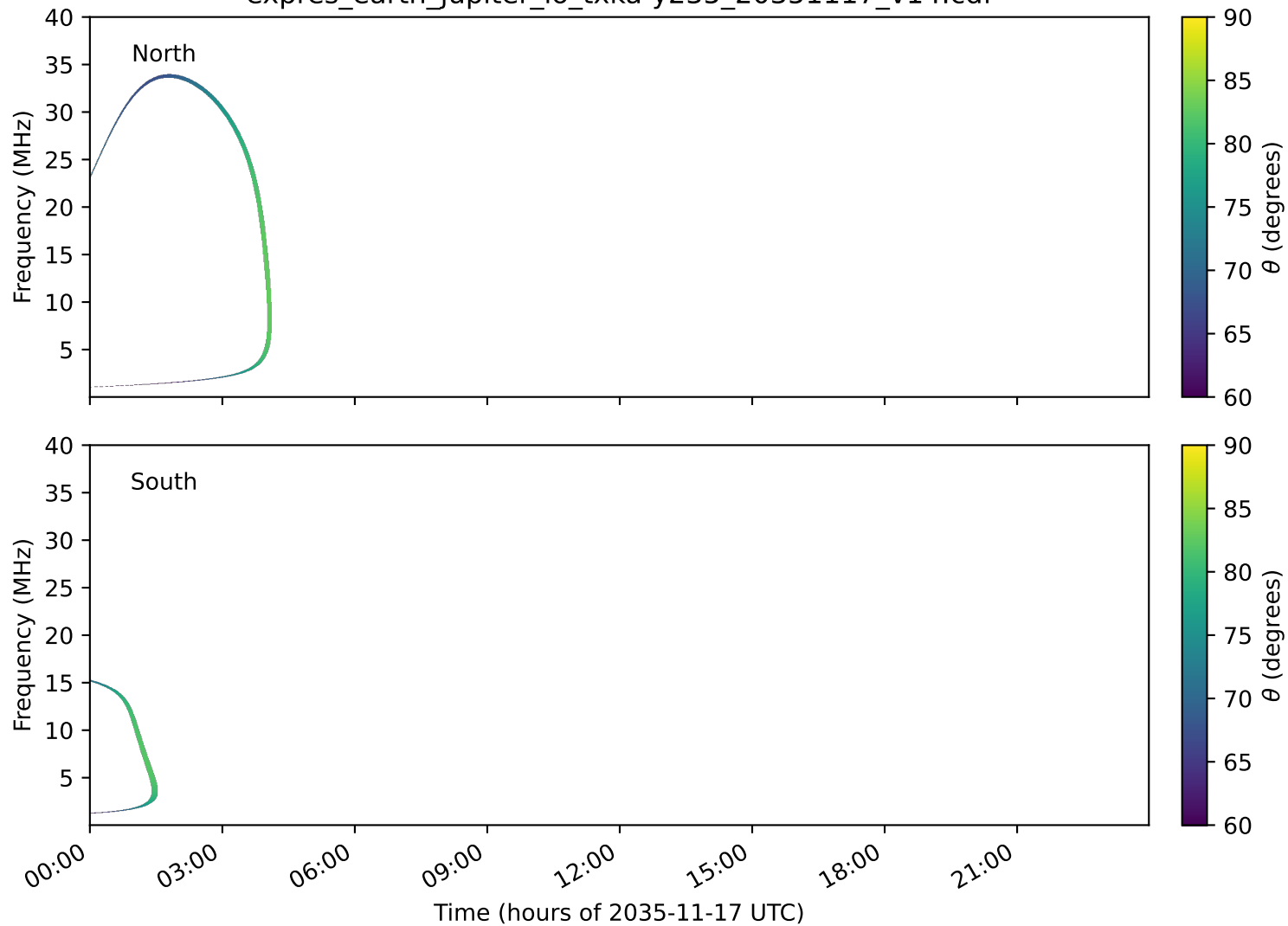
expres_earth_jupiter_io_txka-y235_20351117_v14.cdf
