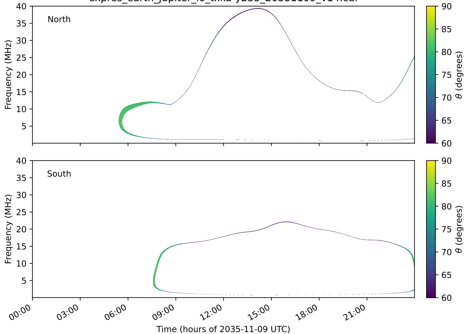
expres_earth_jupiter_io_txka-y235_20351109_v14.cdf
