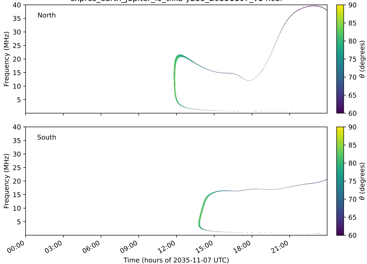
expres_earth_jupiter_io_txka-y235_20351107_v14.cdf
