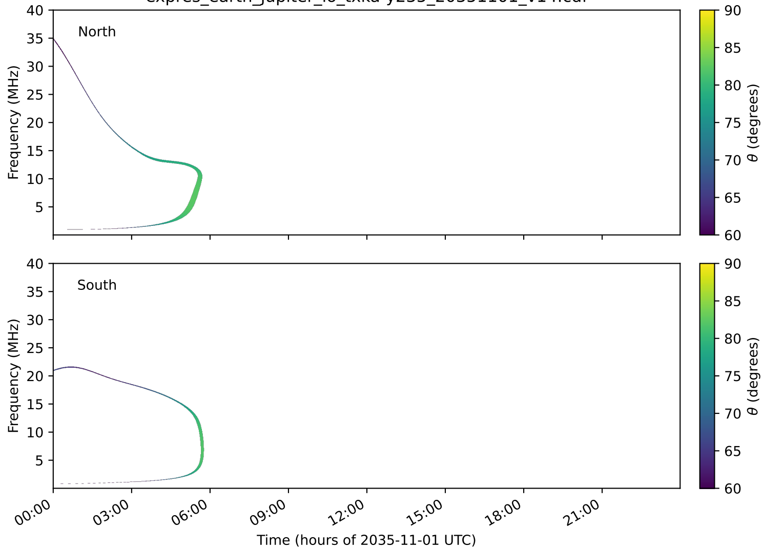
expres_earth_jupiter_io_txka-y235_20351101_v14.cdf
