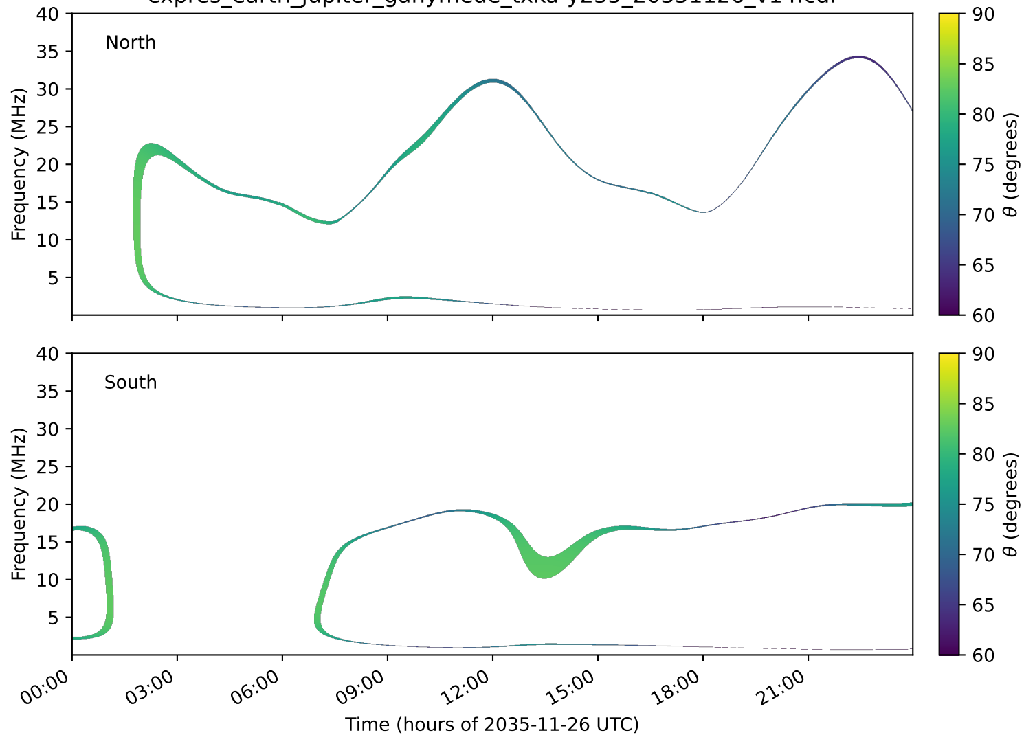
expres_earth_jupiter_ganymede_txka-y235_20351126_v14.cdf
