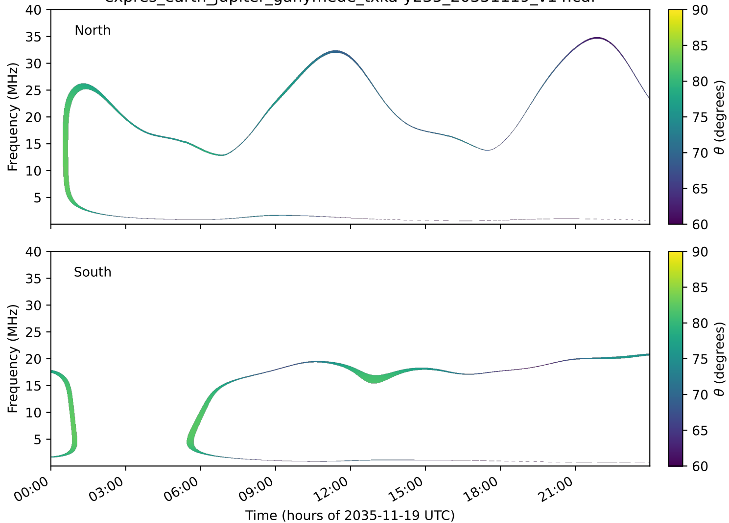
expres_earth_jupiter_ganymede_txka-y235_20351119_v14.cdf
