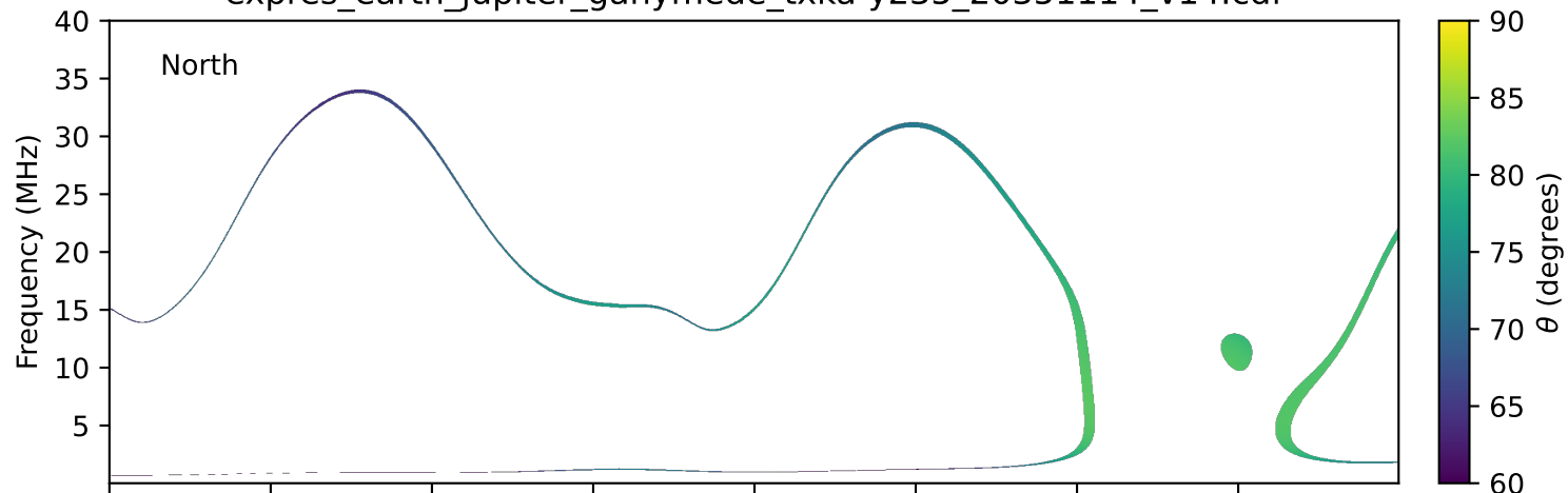
expres_earth_jupiter_ganymede_txka-y235_20351114_v14.cdf
