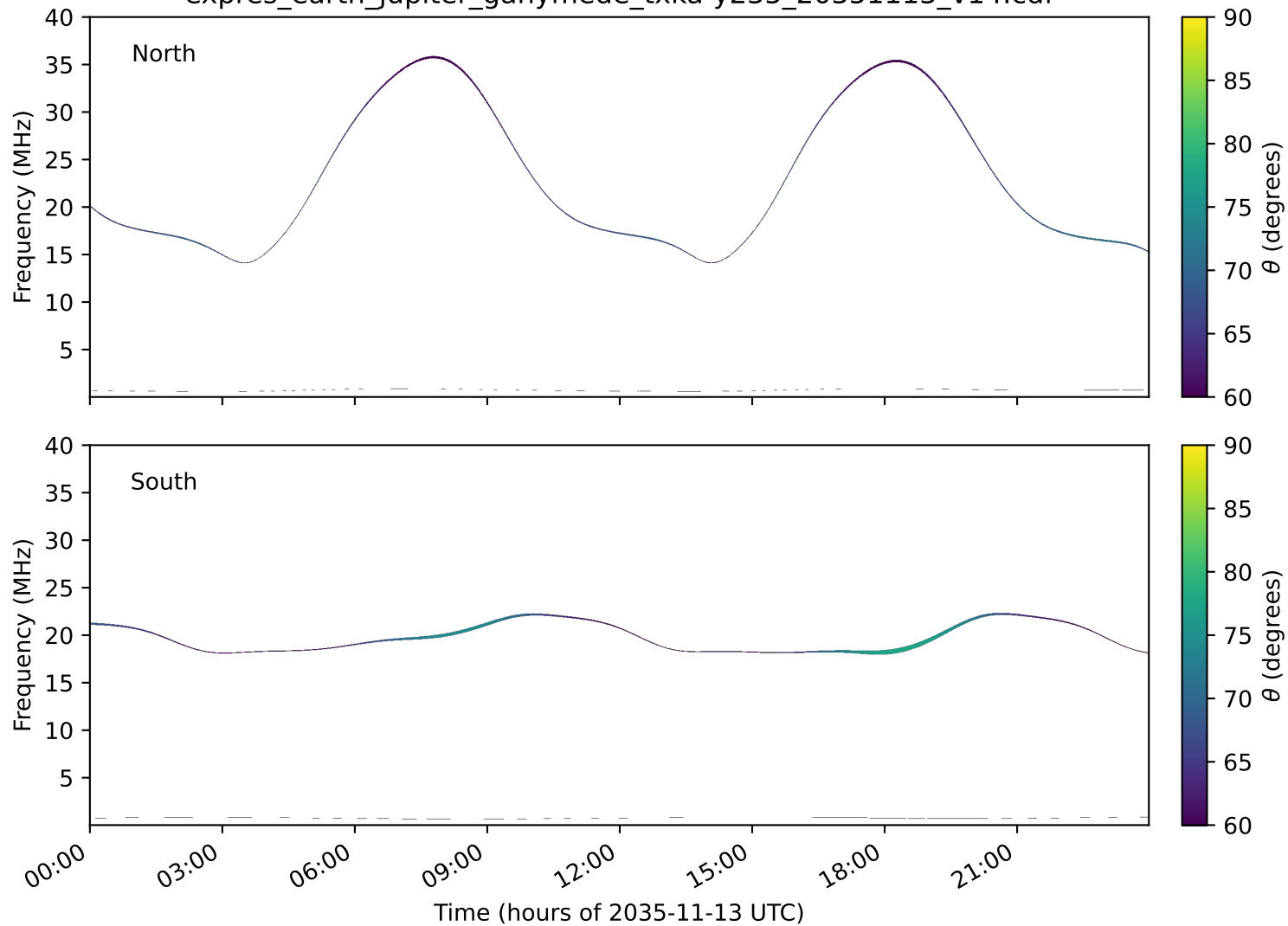
expres_earth_jupiter_ganymede_txka-y235_20351113_v14.cdf
