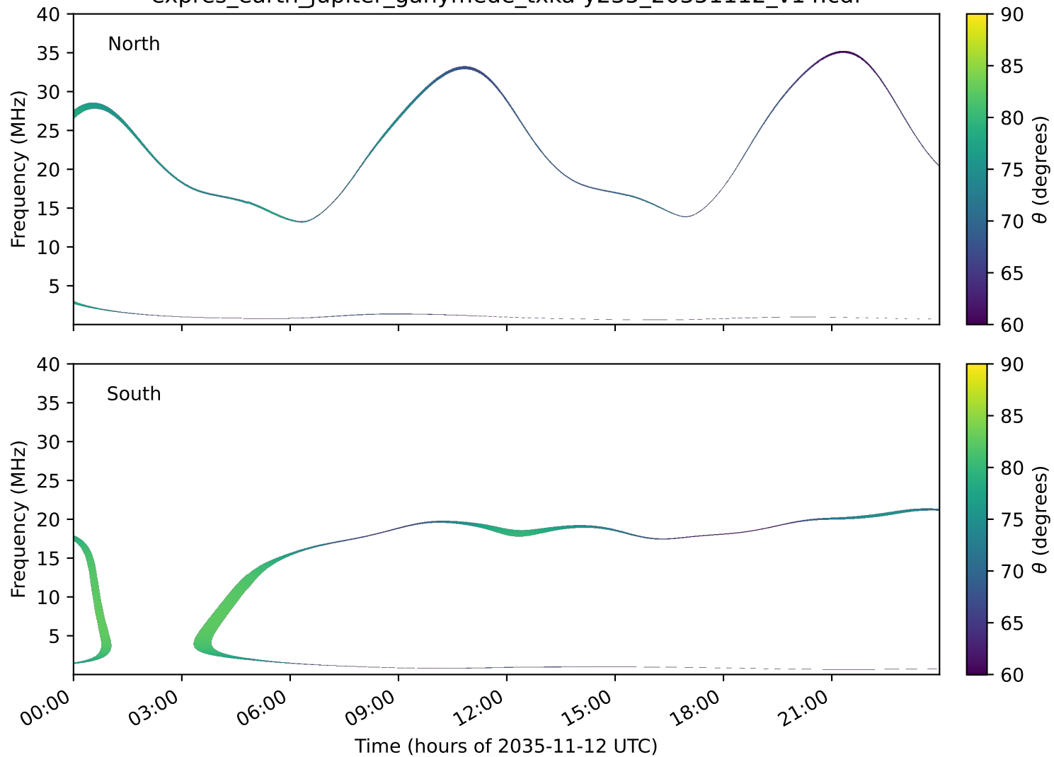
expres_earth_jupiter_ganymede_txka-y235_20351112_v14.cdf
