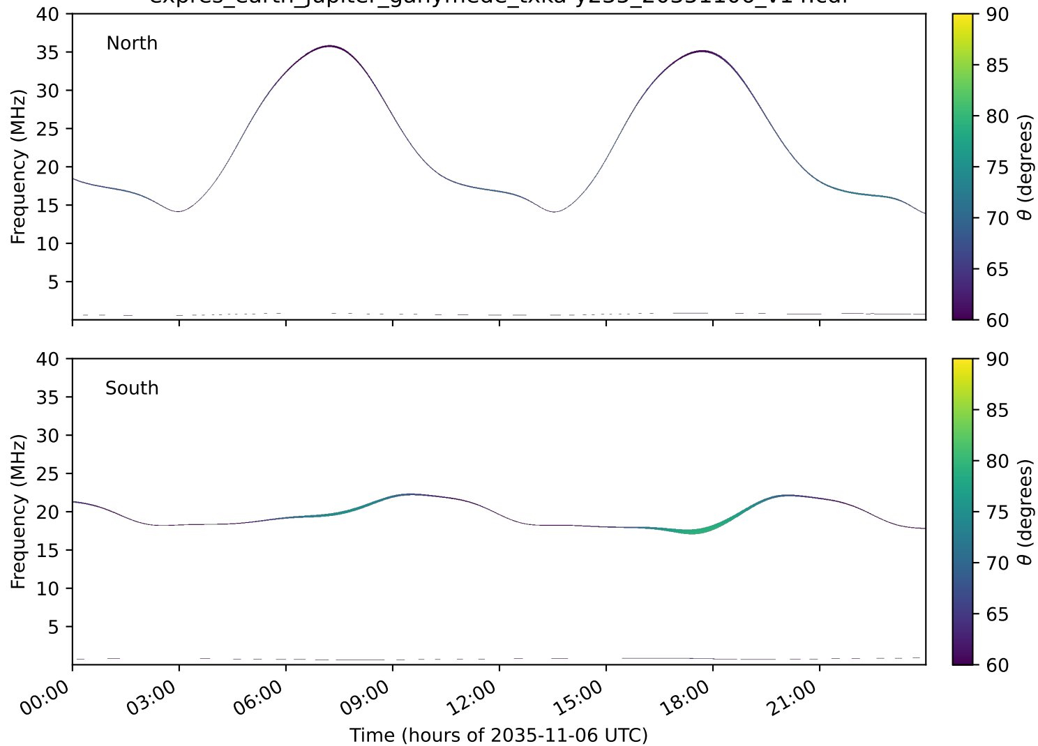
expres_earth_jupiter_ganymede_txka-y235_20351106_v14.cdf
