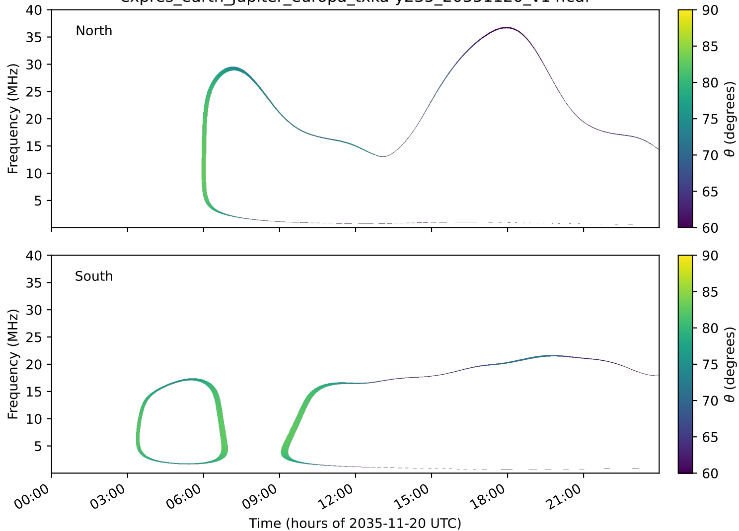
expres_earth_jupiter_europa_txka-y235_20351120_v14.cdf
