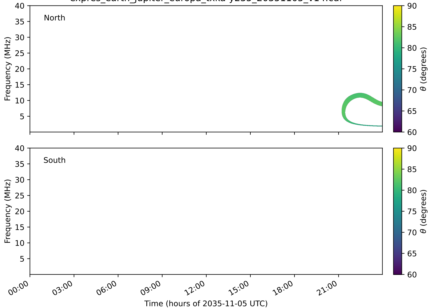
expres_earth_jupiter_europa_txka-y235_20351105_v14.cdf
