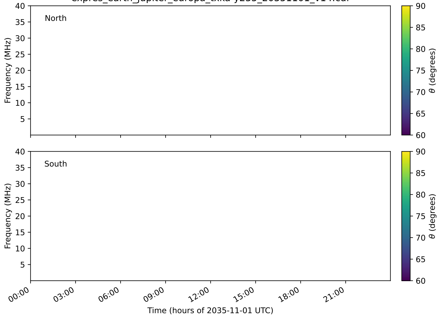
expres_earth_jupiter_europa_txka-y235_20351101_v14.cdf
