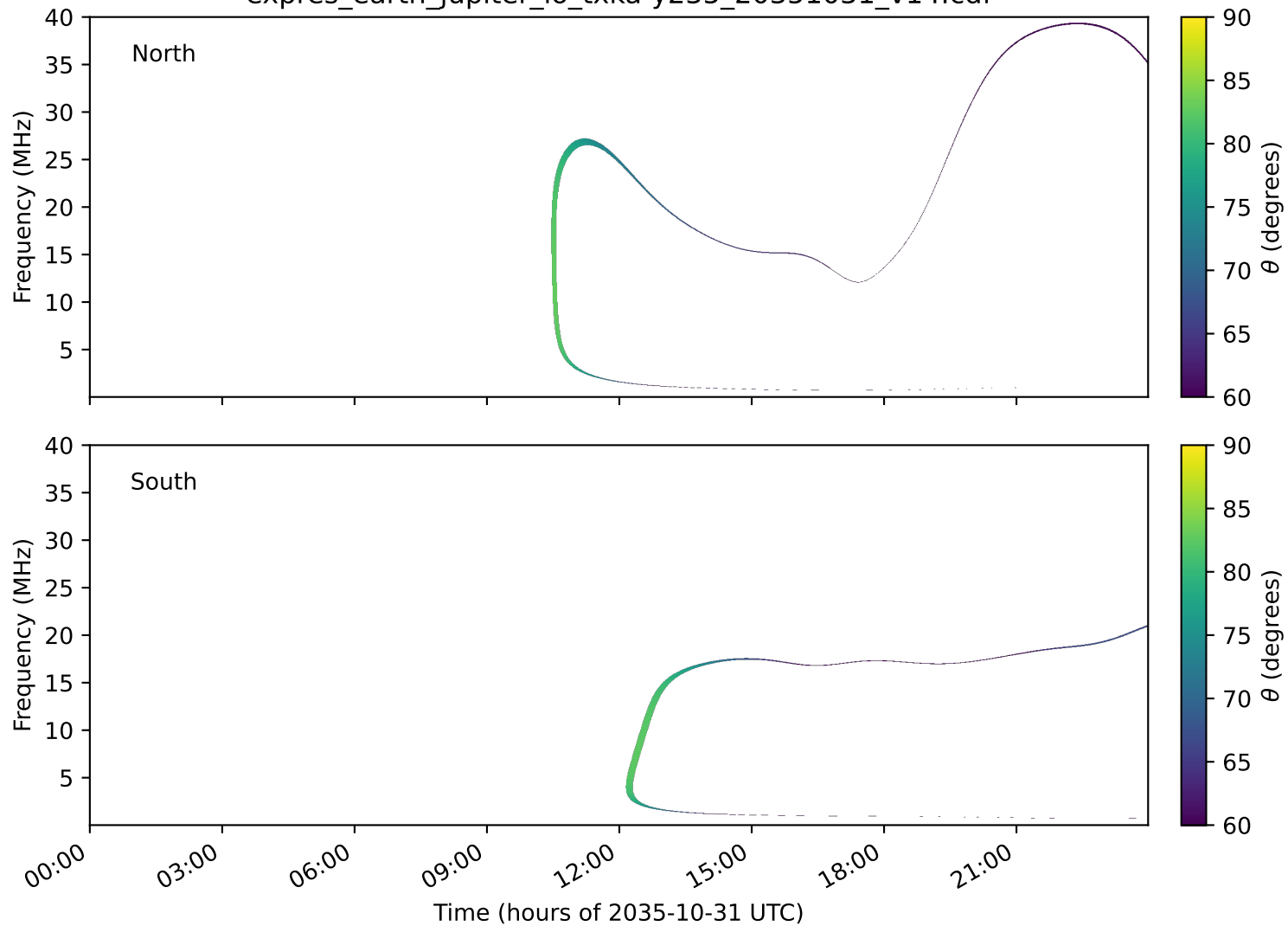
expres_earth_jupiter_io_txka-y235_20351031_v14.cdf
