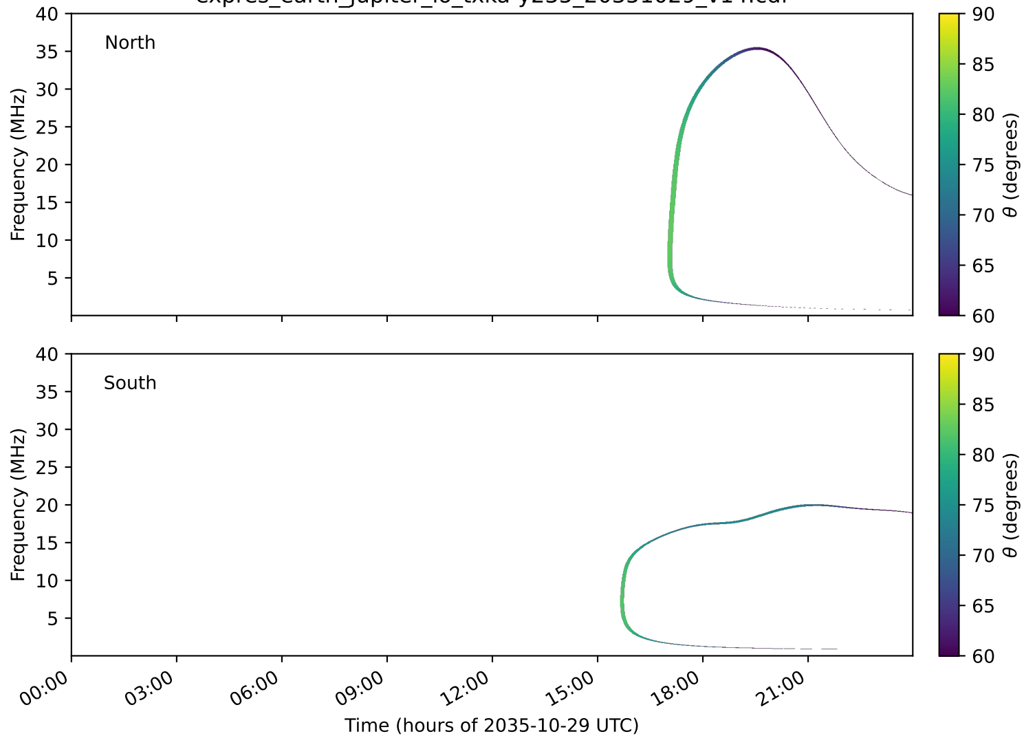
expres_earth_jupiter_io_txka-y235_20351029_v14.cdf
