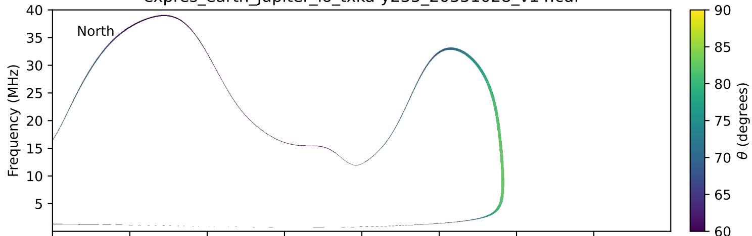
expres_earth_jupiter_io_txka-y235_20351028_v14.cdf
