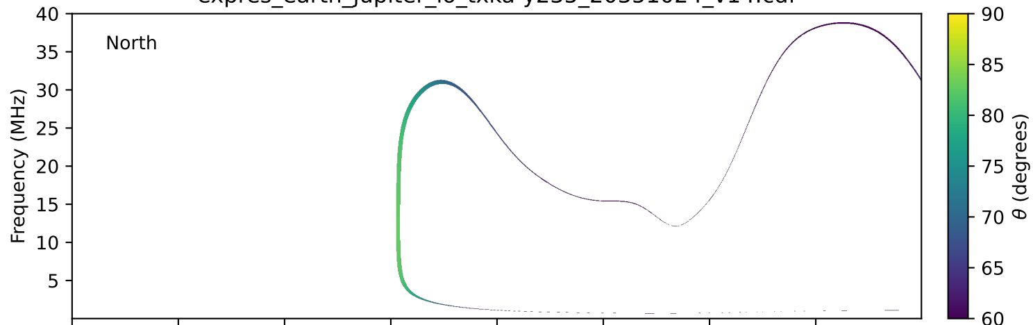
expres_earth_jupiter_io_txka-y235_20351024_v14.cdf
