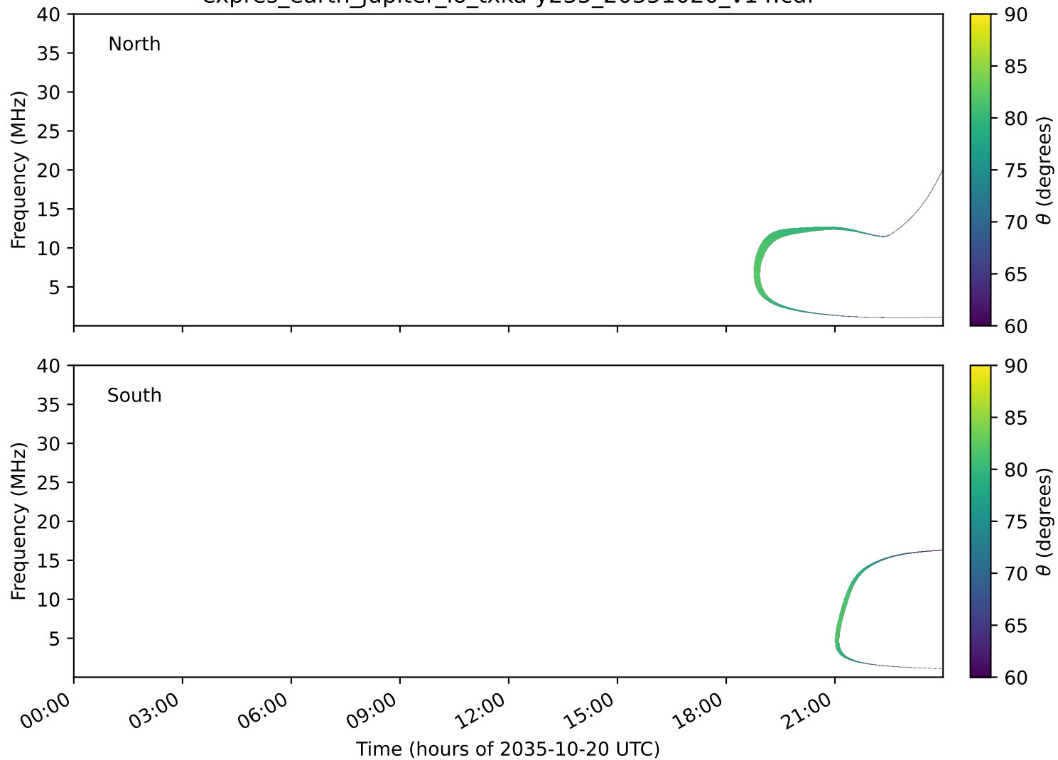
expres_earth_jupiter_io_txka-y235_20351020_v14.cdf
