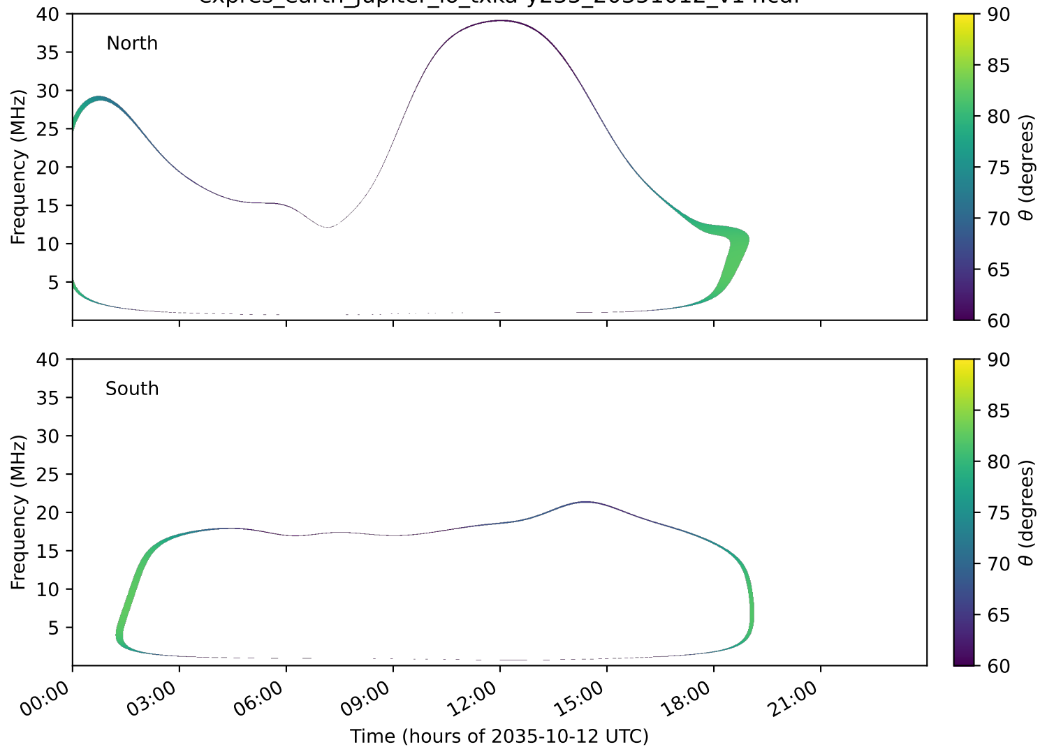
expres_earth_jupiter_io_txka-y235_20351012_v14.cdf
