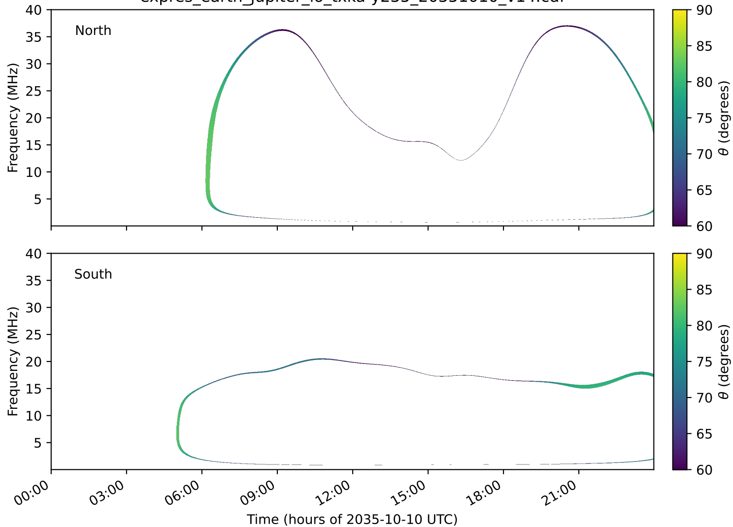
expres_earth_jupiter_io_txka-y235_20351010_v14.cdf
