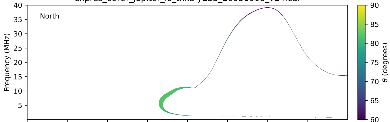
expres_earth_jupiter_io_txka-y235_20351008_v14.cdf
