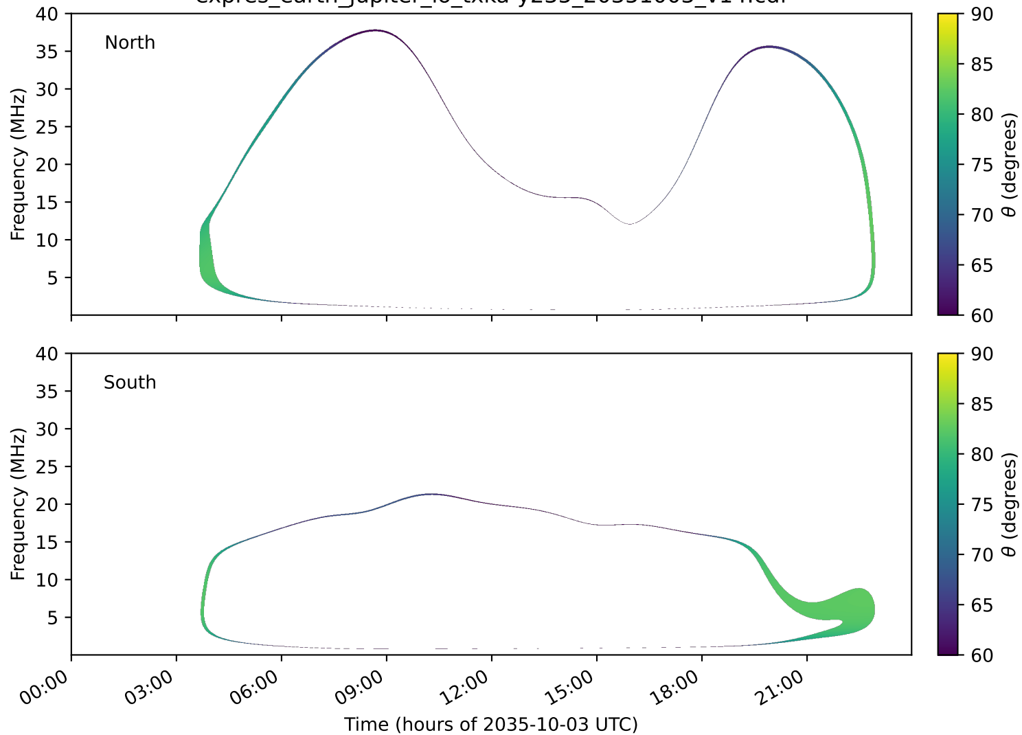
expres_earth_jupiter_io_txka-y235_20351003_v14.cdf
