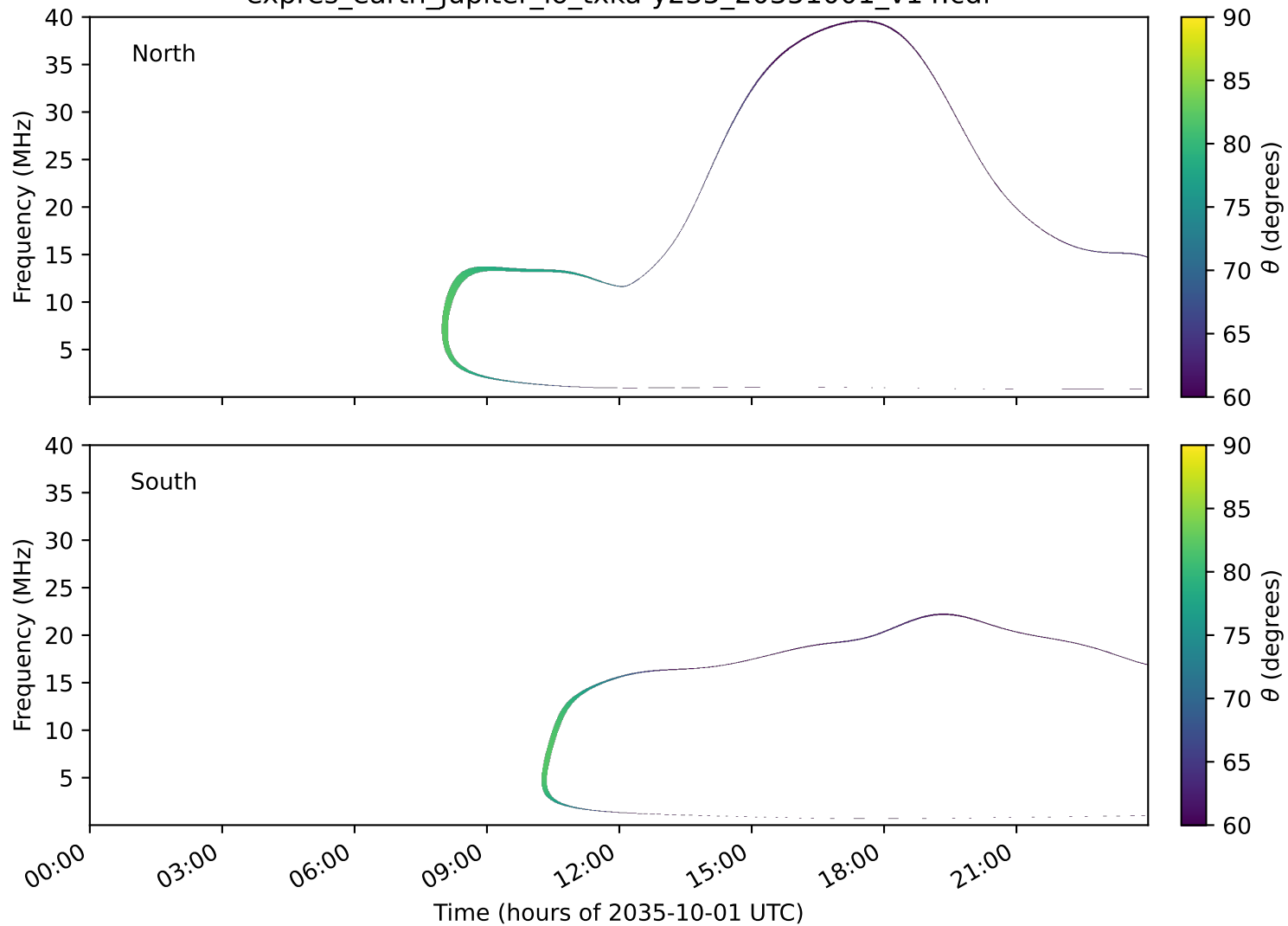
expres_earth_jupiter_io_txka-y235_20351001_v14.cdf
