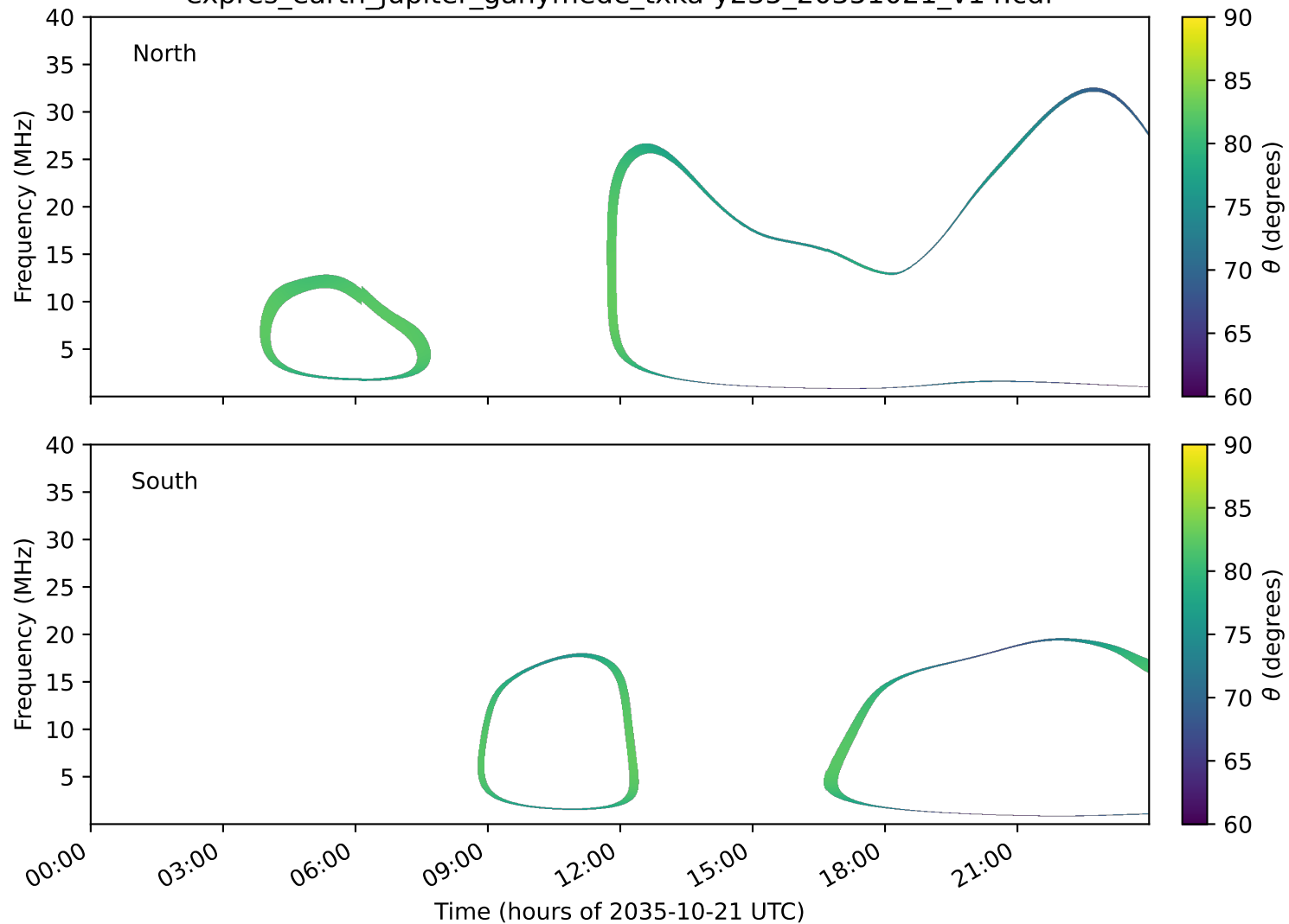
expres_earth_jupiter_ganymede_txka-y235_20351021_v14.cdf
