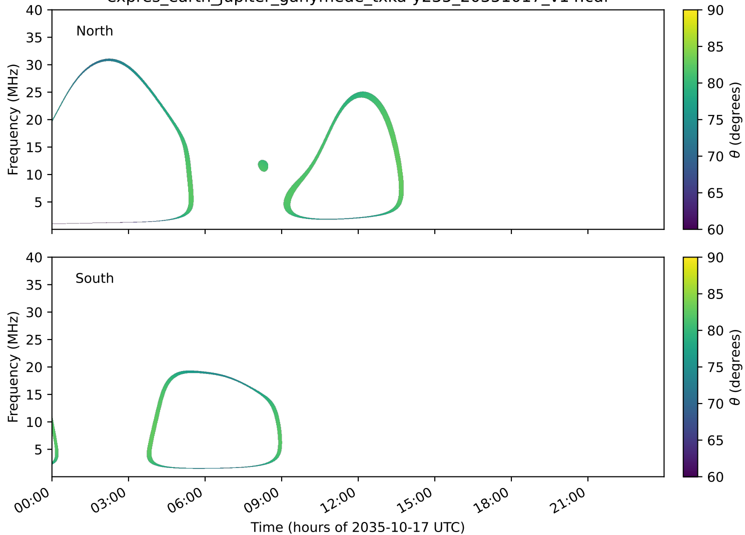
expres_earth_jupiter_ganymede_txka-y235_20351017_v14.cdf
