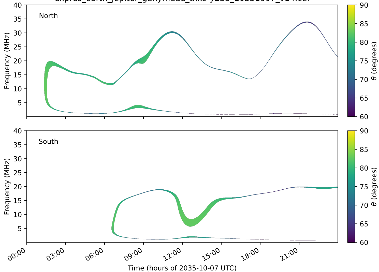
expres_earth_jupiter_ganymede_txka-y235_20351007_v14.cdf
