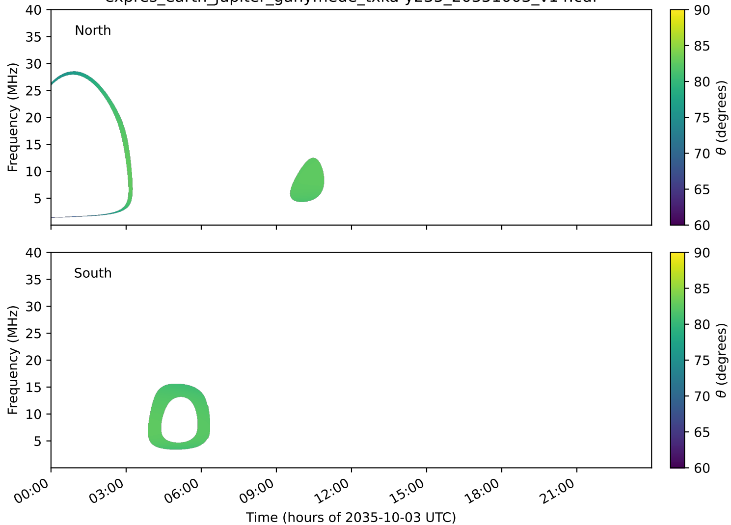
expres_earth_jupiter_ganymede_txka-y235_20351003_v14.cdf
